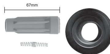
3pc set - Spring Supplied Loose
